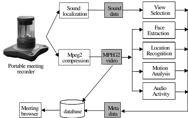
Figure 2. An overview of the meeting recorder system.
