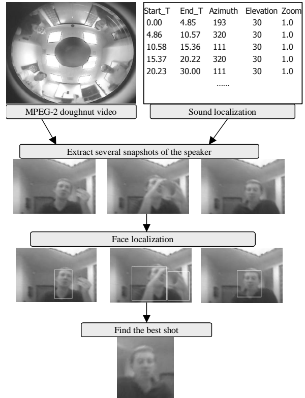
Figure 10. An example of best-shot selection.
