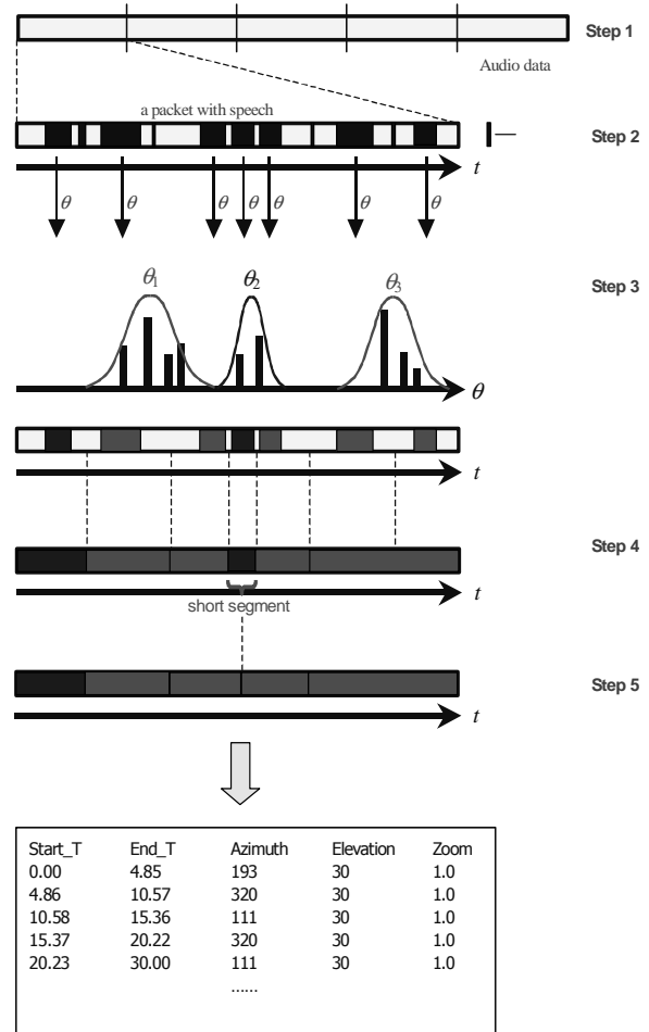
Figure 5. Illustration of the steps in generating view selection metadata. Audio data are divided into blocks of 30 seconds in step 1. Audio segments are grouped in Step 2, followed by clustering in Step 3. Afterward, groups are assigned to clusters.
