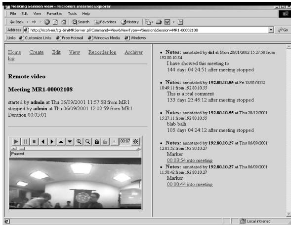
Figure 4. Meeting viewer interface.
