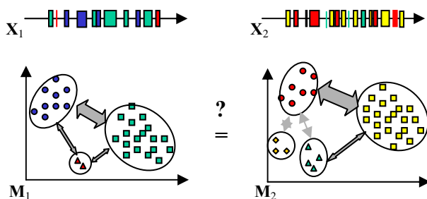
Figure 1 – Meetings are represented by HMMs with a number of speaker states (shade coded) with emission probabilities defined over feature space, and transition probabilities (shown as arrows) among the states. Meeting similarity is determined by comparing two HMMs.
